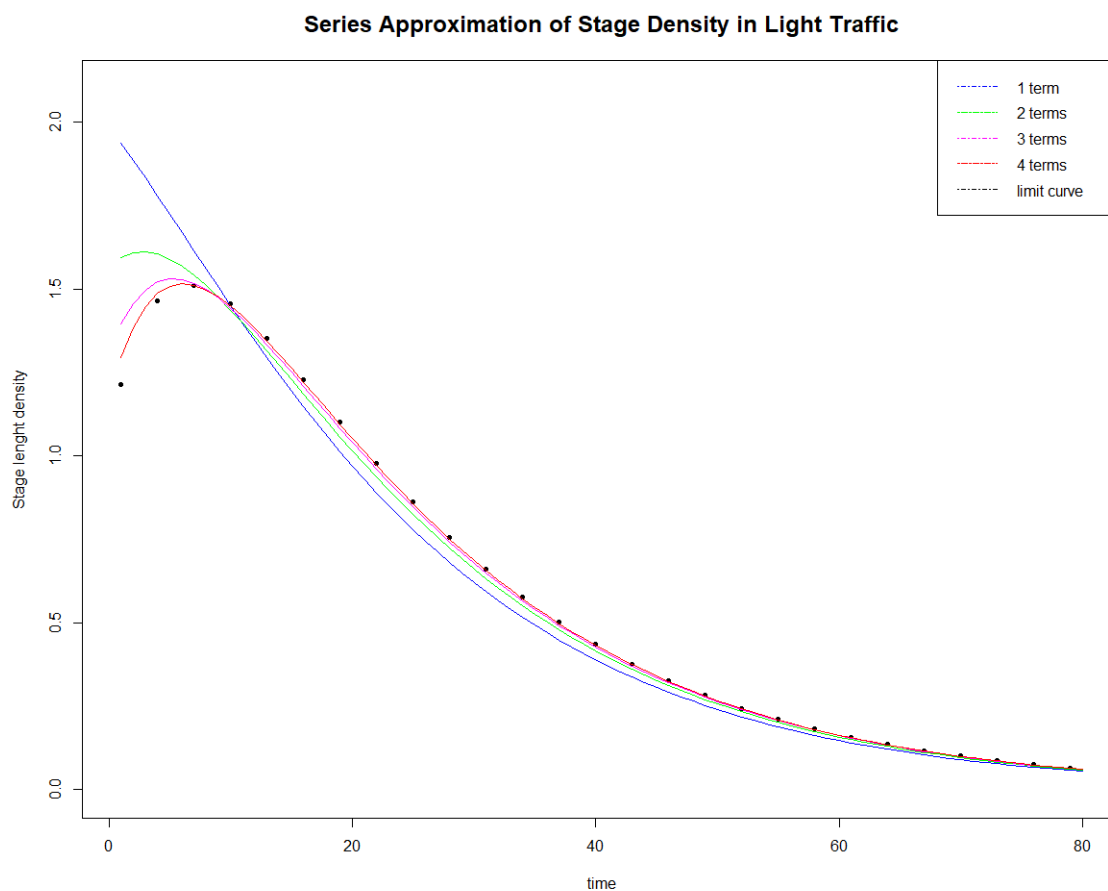
Fig. 3.1: A series representation for the stationary density of the length of a stage in a gated M/G/\infty queue in light traffic.
